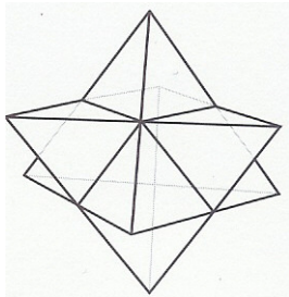
afb. ster-tetraëder
